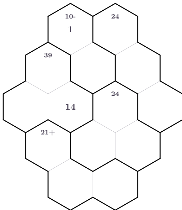
Hex Math Path 7
